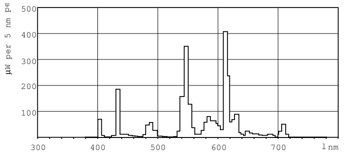
LDPB_PLS4PLM_830-Spectral power distribution B/W
