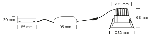
*The drawing is not drawn to scale
