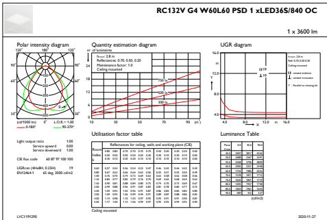
IFGU1_RC132VG4W60L60PSD1xLED36S840OC
