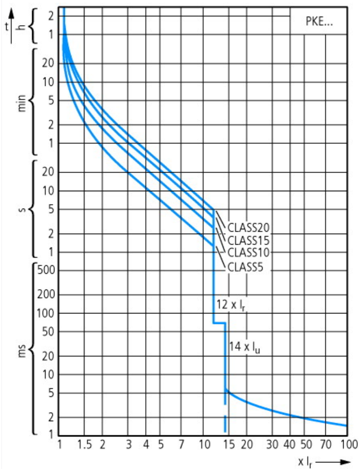
Tripping characteristics
